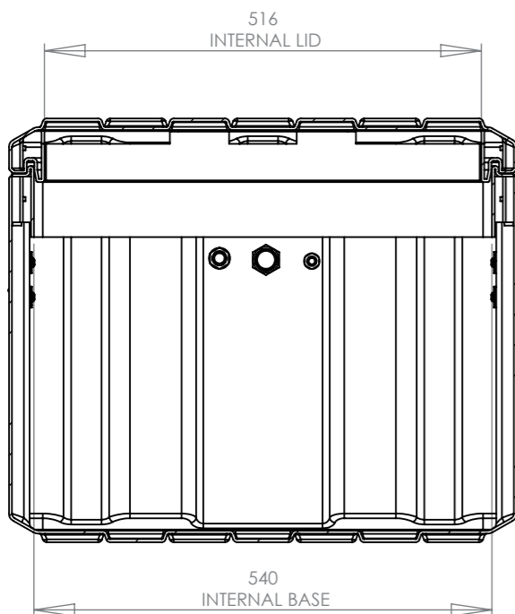
SECTION Y-Y SCALE 1 : 8
