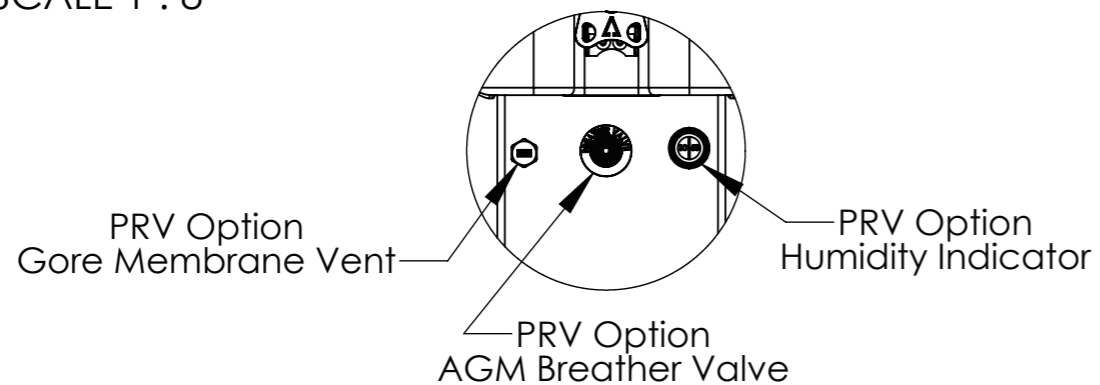
SECTION Y-Y SCALE 1 : 8
