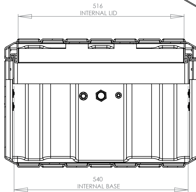
SECTION Y-Y SCALE 1 : 7
