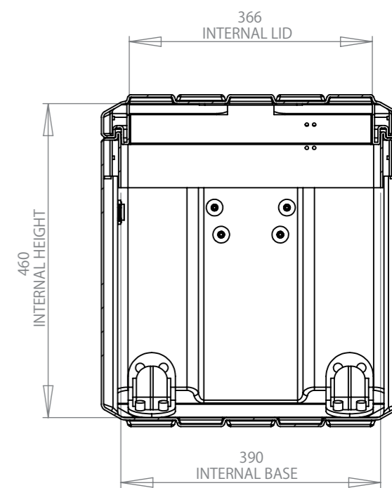
SECTION Z-Z SCALE 1 : 8
