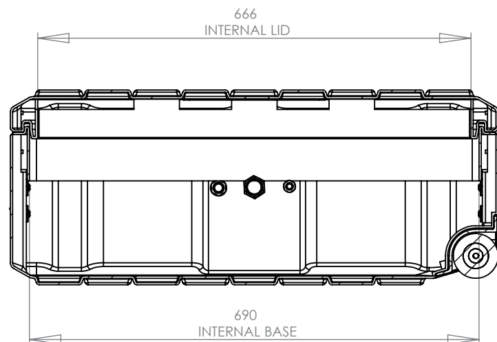
SECTION Y-Y SCALE 1 : 8
