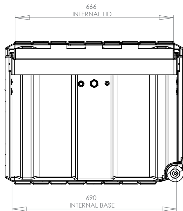
SECTION Y-Y
