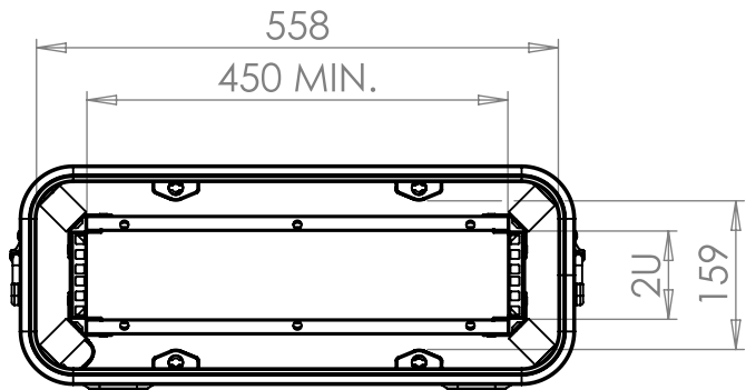
VIEW B SHOWING CASE WITH LIDS REMOVED
