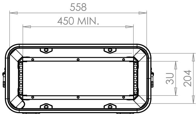
VIEW B SHOWING CASE WITH LIDS REMOVED
