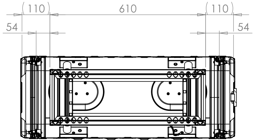
SECTION A-A SHOWING CHASSIS DETAIL
