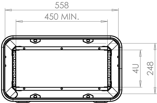
VIEW B SHOWING CASE WITH LIDS REMOVED
