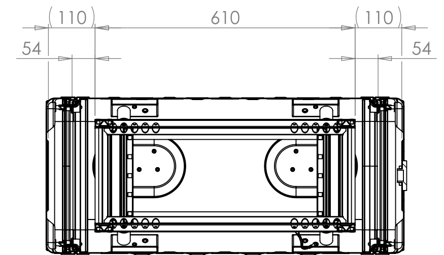
SECTION A-A SHOWING CHASSIS DETAIL
