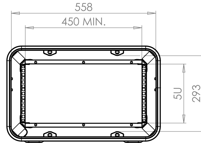
VIEW B SHOWING CASE WITH LIDS REMOVED
