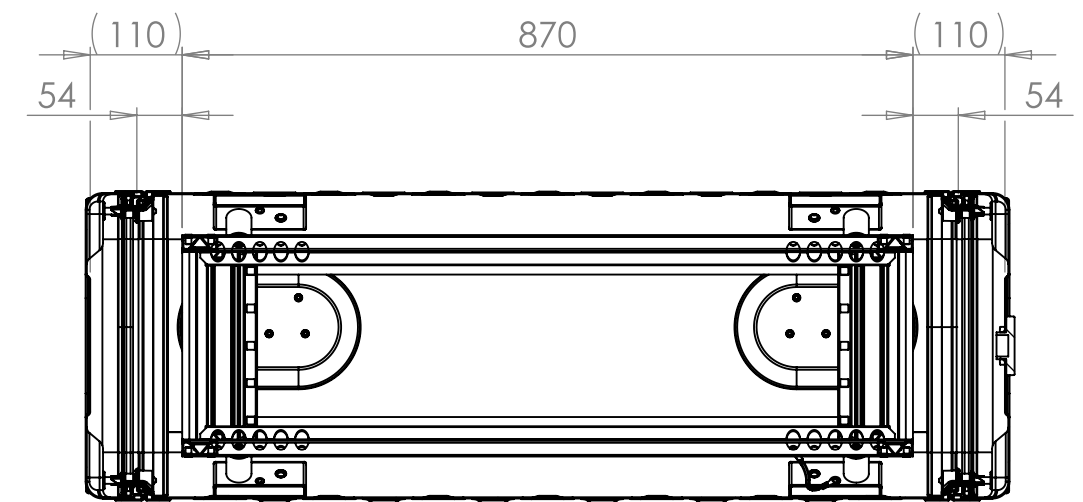
SECTION A-A SHOWING CHASSIS DETAIL
