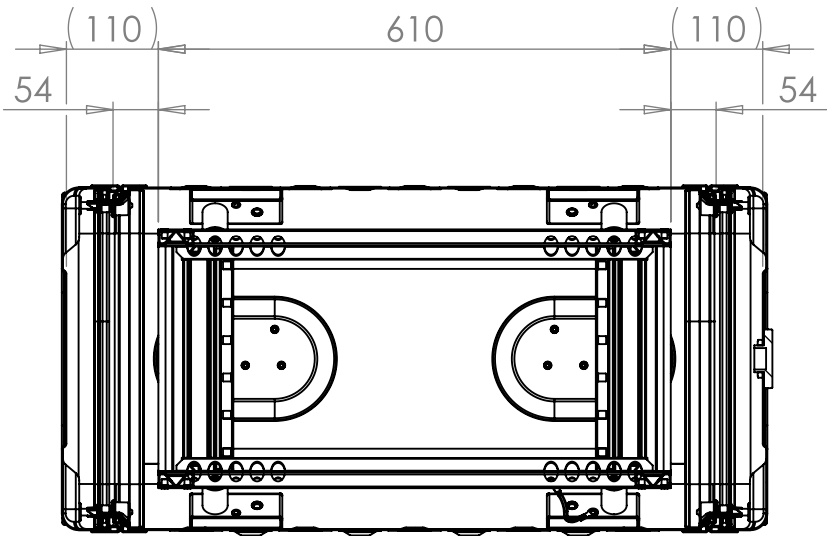
SECTION A-A SHOWING CHASSIS DETAIL
