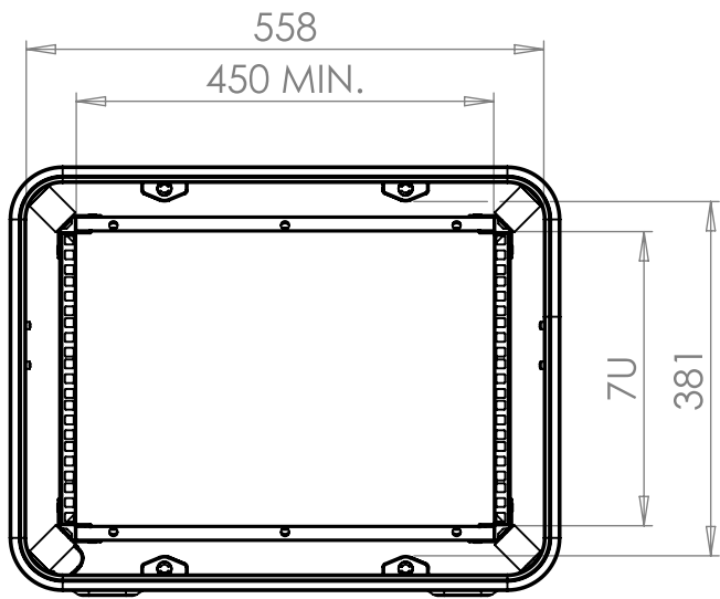
VIEW B SHOWING CASE WITH LIDS REMOVED
