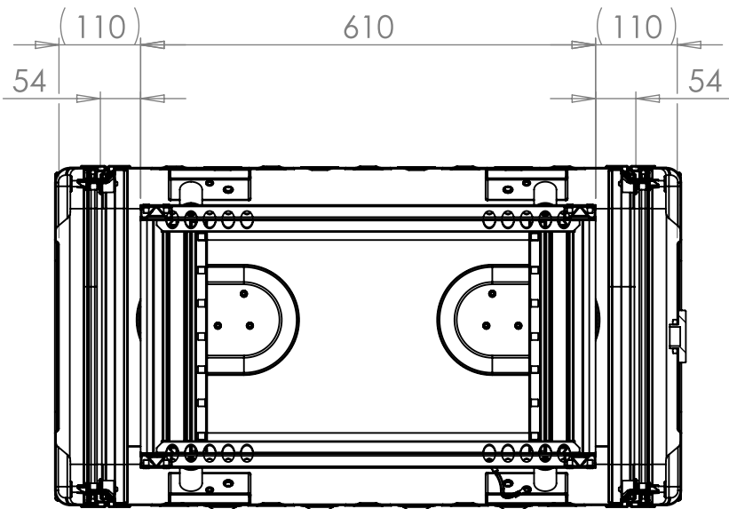
SECTION A-A SHOWING CHASSIS DETAIL
