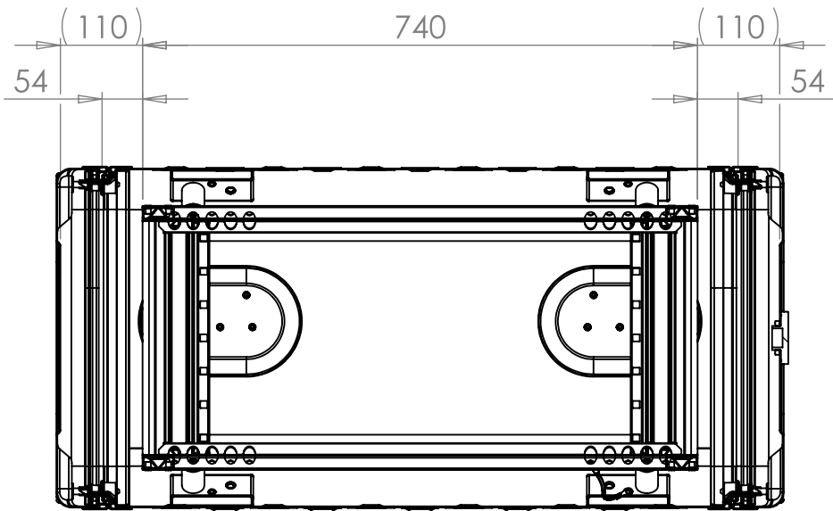
SECTION A-A SHOWING CHASSIS DETAIL
