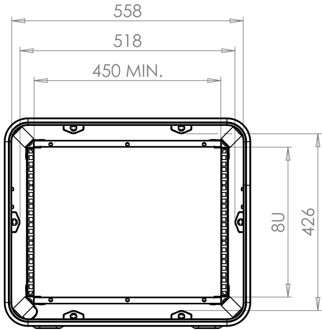
VIEW B SHOWING CASE WITH LIDS REMOVED
