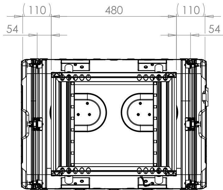
SECTION A-A SHOWING CHASSIS DETAIL
