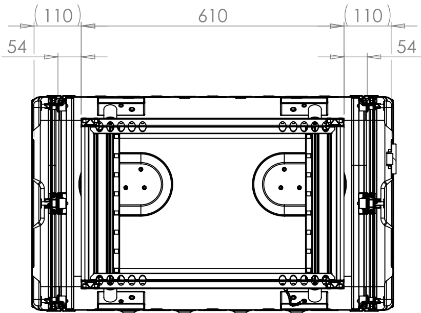
SECTION A-A SHOWING CHASSIS DETAIL
