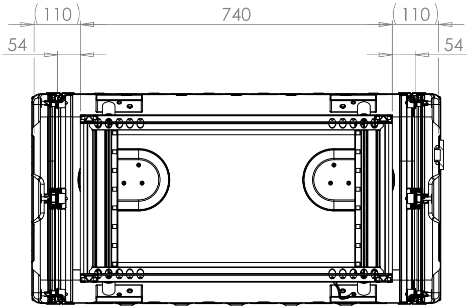
SECTION A-A SHOWING CHASSIS DETAIL
