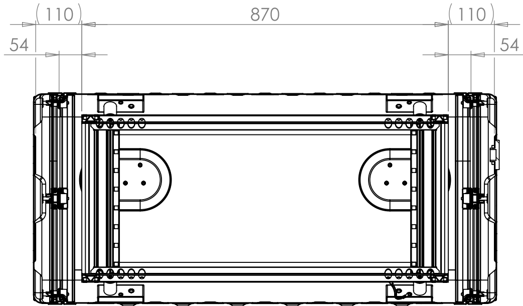
SECTION A-A SHOWING CHASSIS DETAIL
