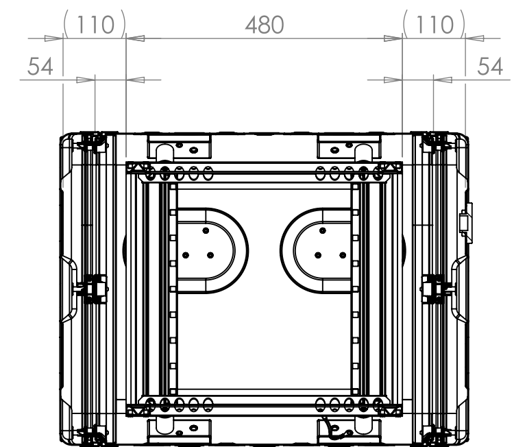
SECTION A-A SHOWING CHASSIS DETAIL
