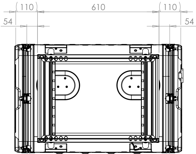
SECTION A-A SHOWING CHASSIS DETAIL
