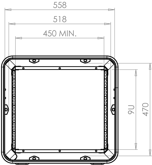
VIEW B SHOWING CASE WITH LIDS REMOVED
