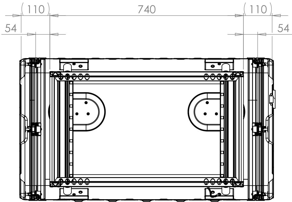
SECTION A-A SHOWING CHASSIS DETAIL
