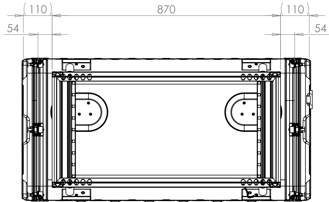
SECTION A-A SHOWING CHASSIS DETAIL
