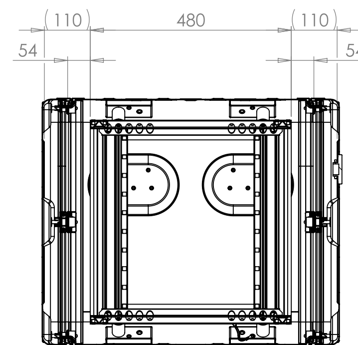
SECTION A-A SHOWING CHASSIS DETAIL
