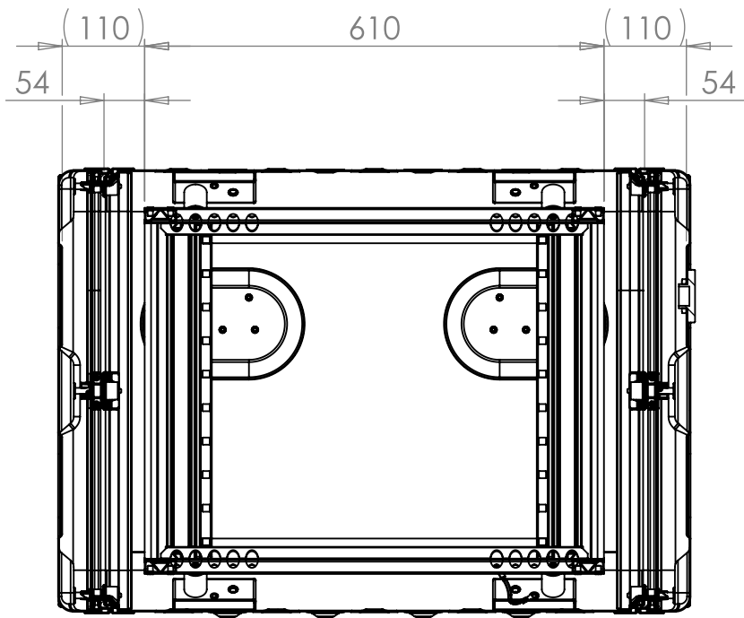
SECTION A-A SHOWING CHASSIS DETAIL
