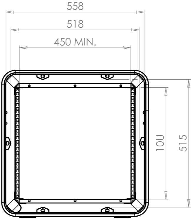
VIEW B SHOWING CASE WITH LIDS REMOVED
