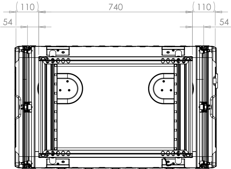
SECTION A-A SHOWING CHASSIS DETAIL
