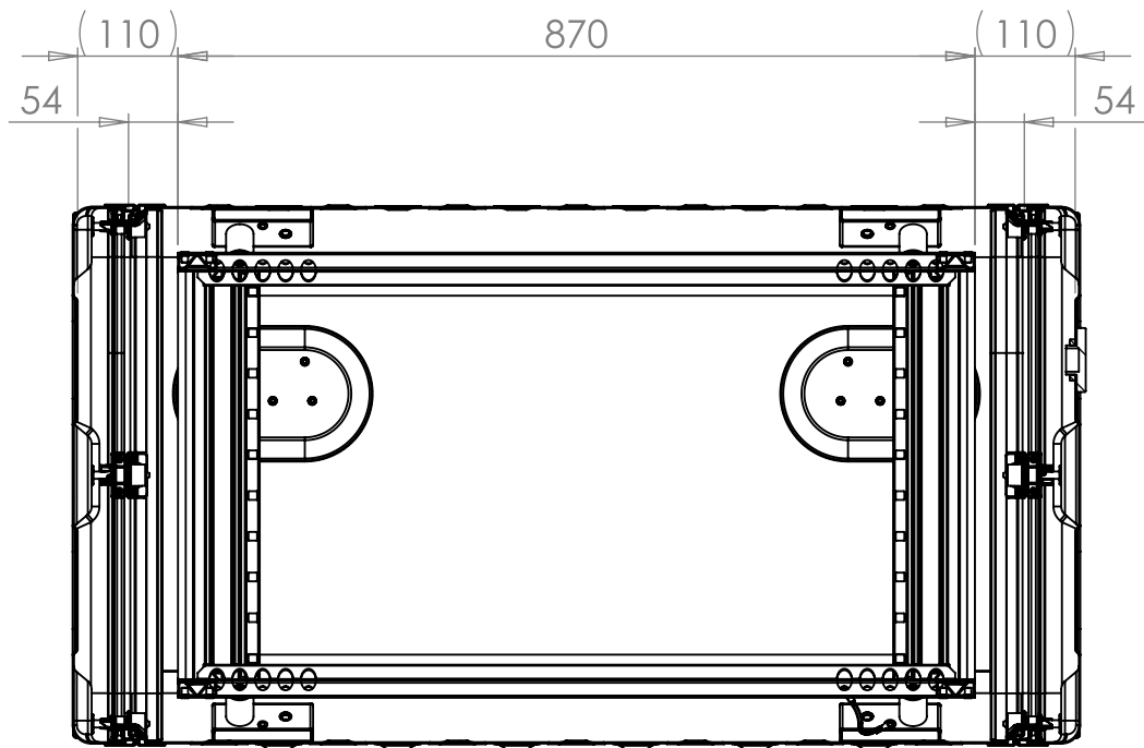
SECTION A-A SHOWING CHASSIS DETAIL
