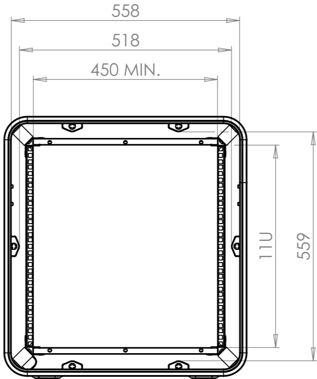
VIEW B SHOWING CASE WITH LIDS REMOVED
