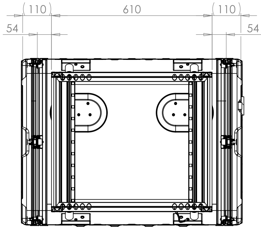
SECTION A-A SHOWING CHASSIS DETAIL
