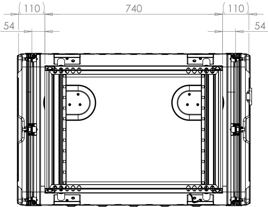
SECTION A-A SHOWING CHASSIS DETAIL
