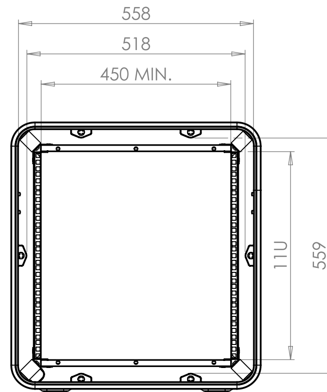
VIEW B SHOWING CASE WITH LIDS REMOVED
