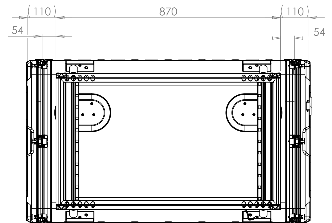
SECTION A-A SHOWING CHASSIS DETAIL
