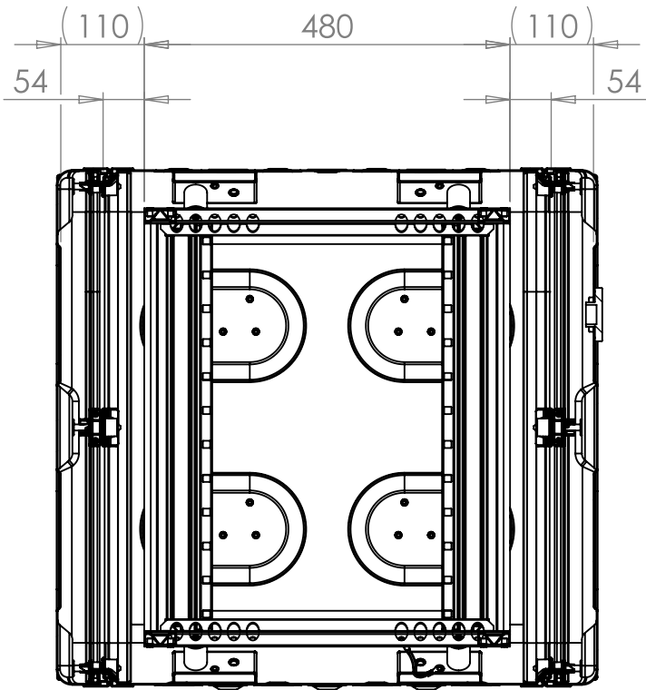
SECTION A-A SHOWING CHASSIS DETAIL
