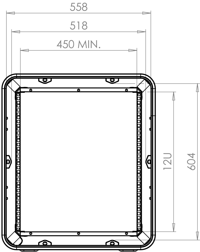
VIEW B SHOWING CASE WITH LIDS REMOVED
