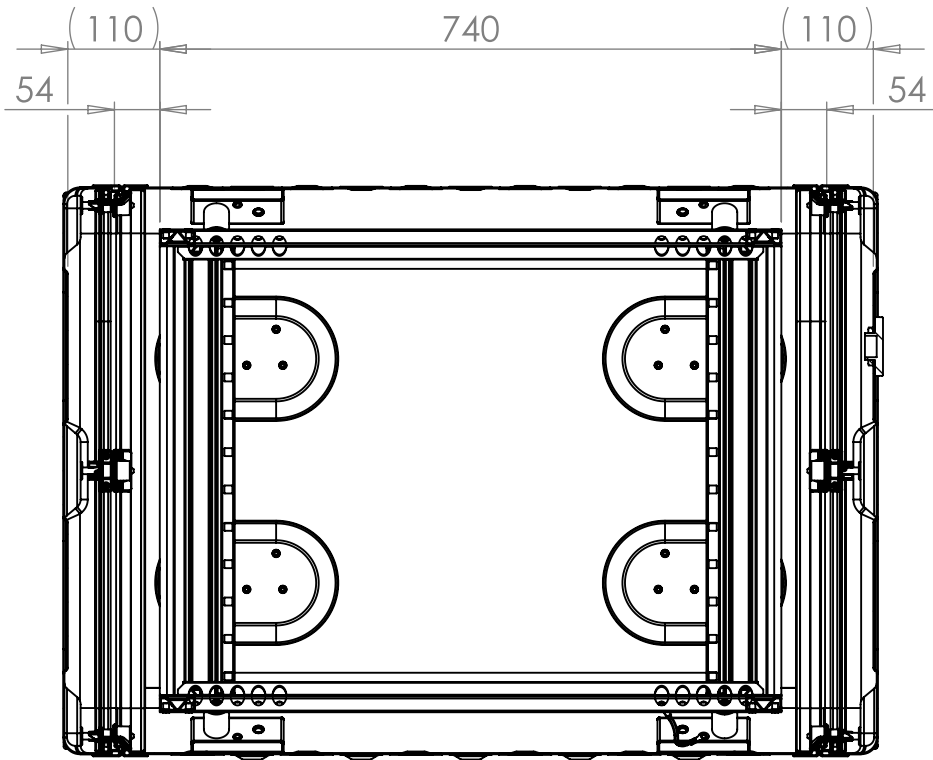
SECTION A-A SHOWING CHASSIS DETAIL
