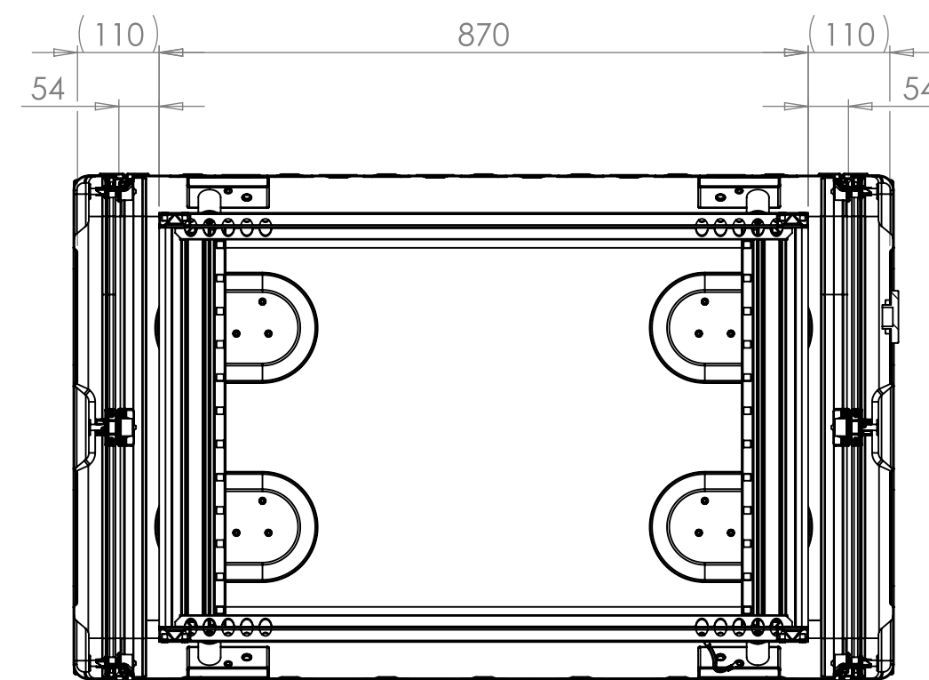
SECTION A-A SHOWING CHASSIS DETAIL
