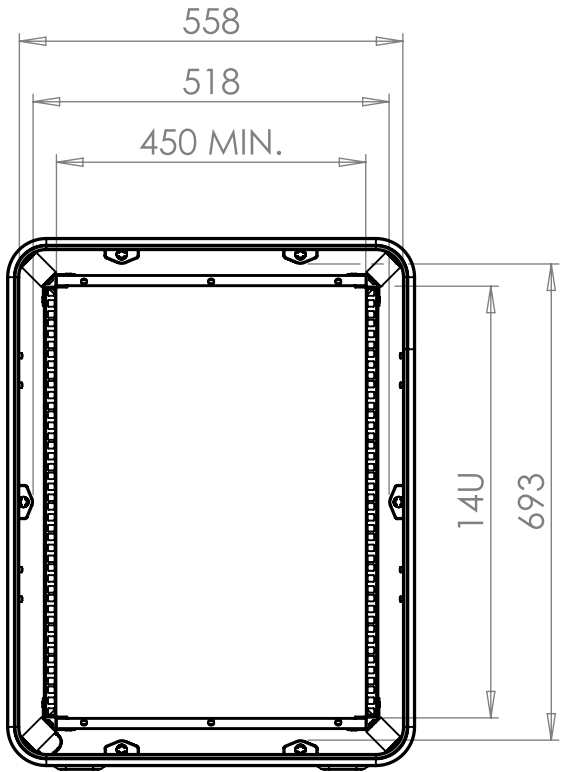
VIEW B SHOWING CASE WITH LIDS REMOVED
