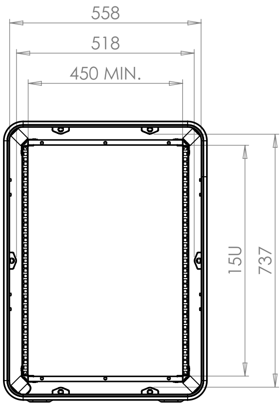
VIEW B SHOWING CASE WITH LIDS REMOVED
