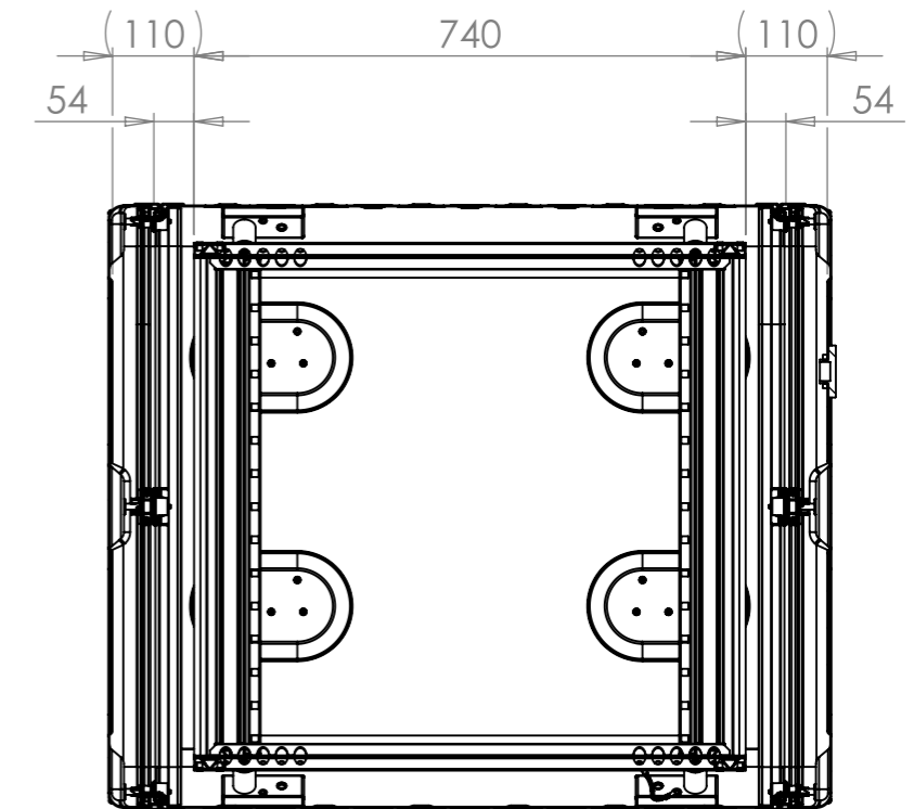
SECTION A-A SHOWING CHASSIS DETAIL
