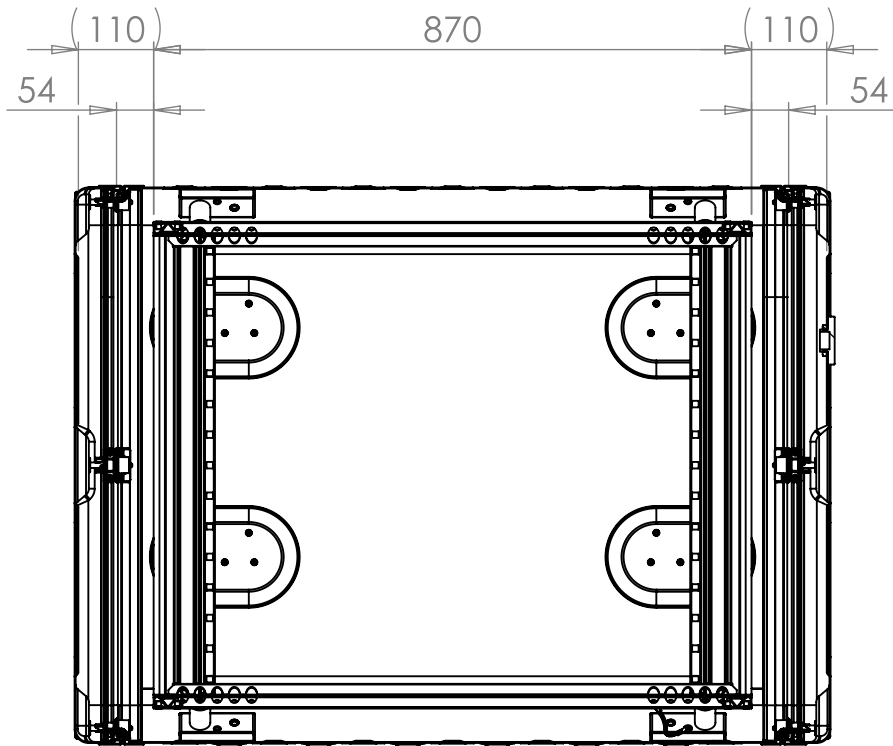
SECTION A-A SHOWING CHASSIS DETAIL
