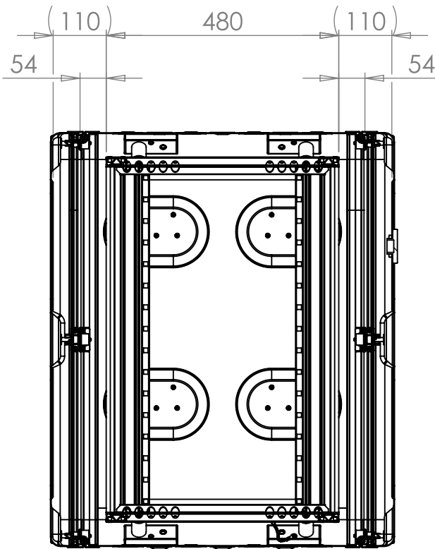
SECTION A-A SHOWING CHASSIS DETAIL
