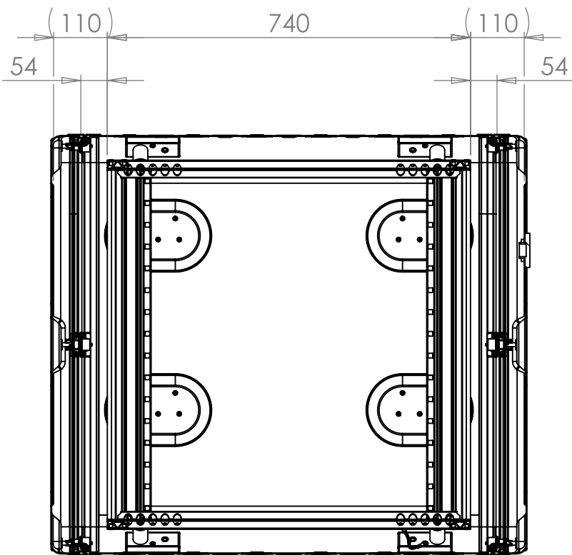
SECTION A-A SHOWING CHASSIS DETAIL
