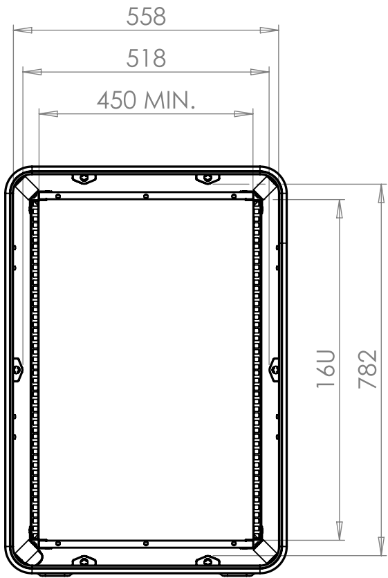
VIEW B SHOWING CASE WITH LIDS REMOVED
