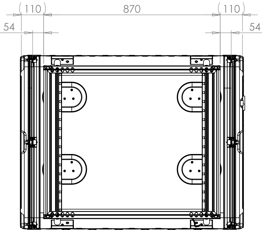
SECTION A-A SHOWING CHASSIS DETAIL
