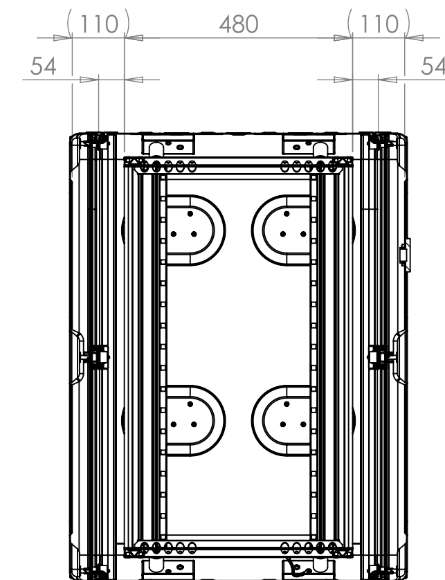
SECTION A-A SHOWING CHASSIS DETAIL
