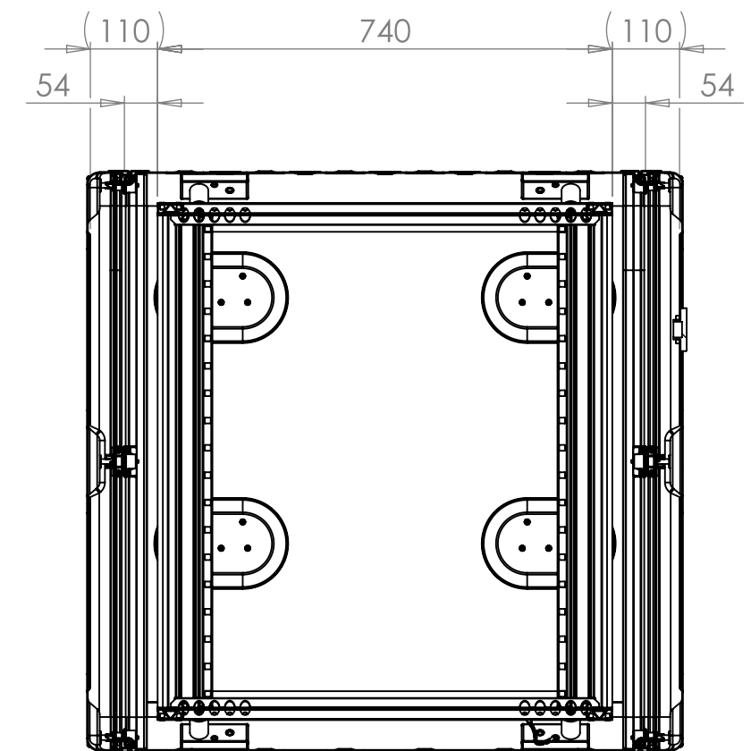
SECTION A-A SHOWING CHASSIS DETAIL
