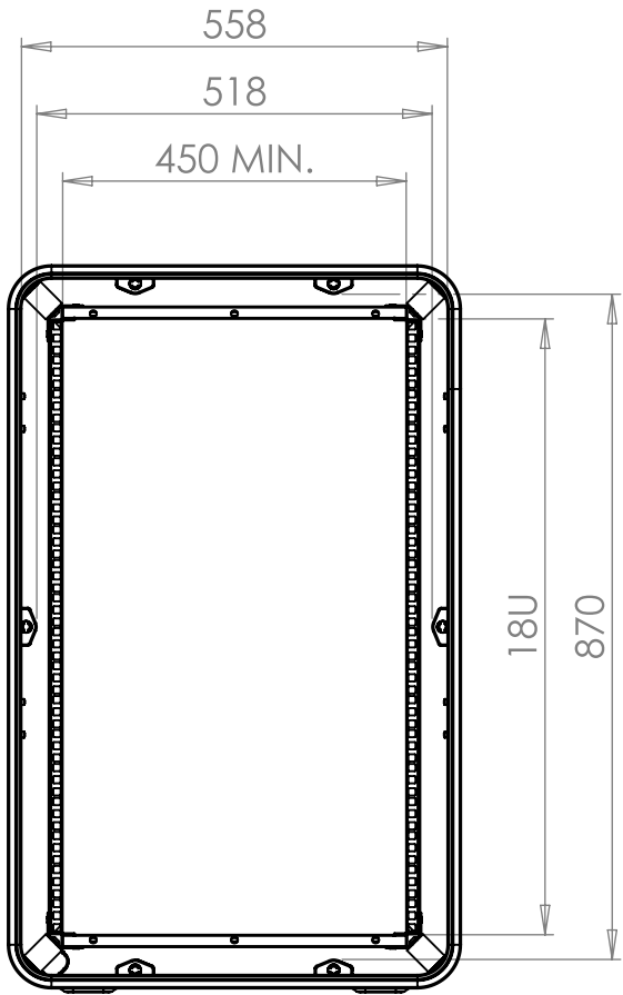
VIEW B SHOWING CASE WITH LIDS REMOVED
