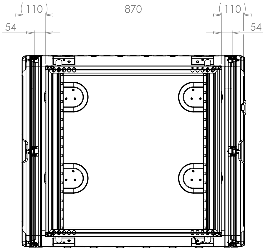
SECTION A-A SHOWING CHASSIS DETAIL
